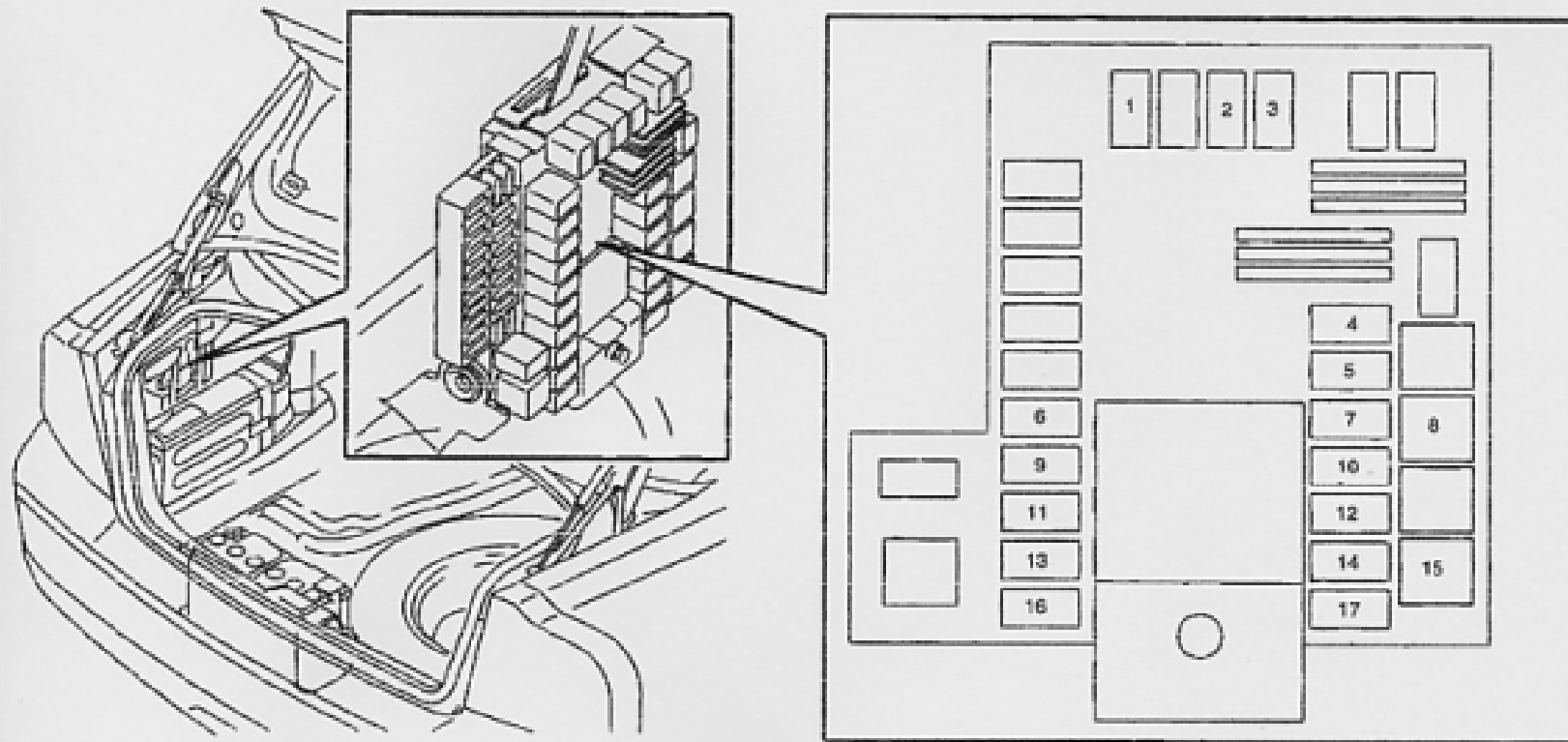
ELECTRICAL COMPONENT LOCATOR Fig. 6: Cargo Compartment Relay/Fuse Box Courtesy of Volvo Cars of North America. 2001 Volvo S80
